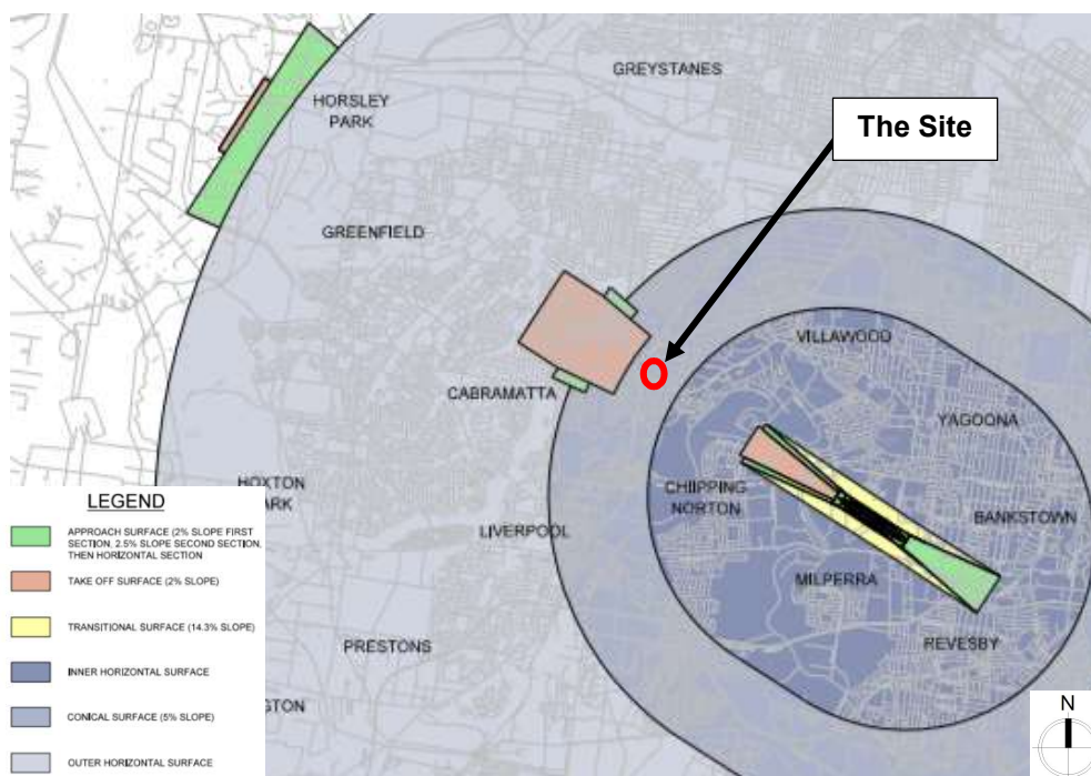
Figure 15: Obstacle limitation surfaces for Bankstown Airport.
